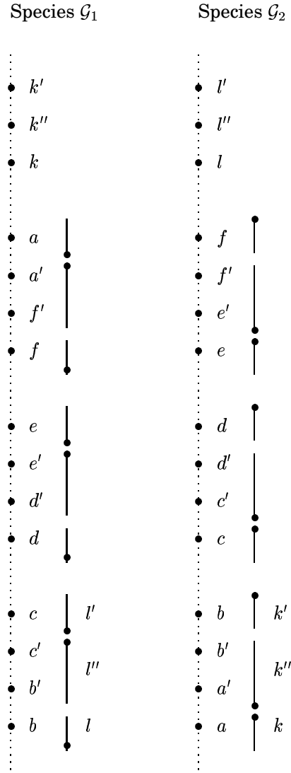
Figure 2: Depth 2 gene arrangement: a cyclic structure with two optimal solutions. The alternative optimal solution is obtained by moving all the non-fixed genes to the opposite ends of their intervals. (Note that only two of the six 7-units are depicted in full; the unlabelled genes whose positions are not fixed correspond to sequences of three consecutive fixed genes (not shown) on the other species.)
