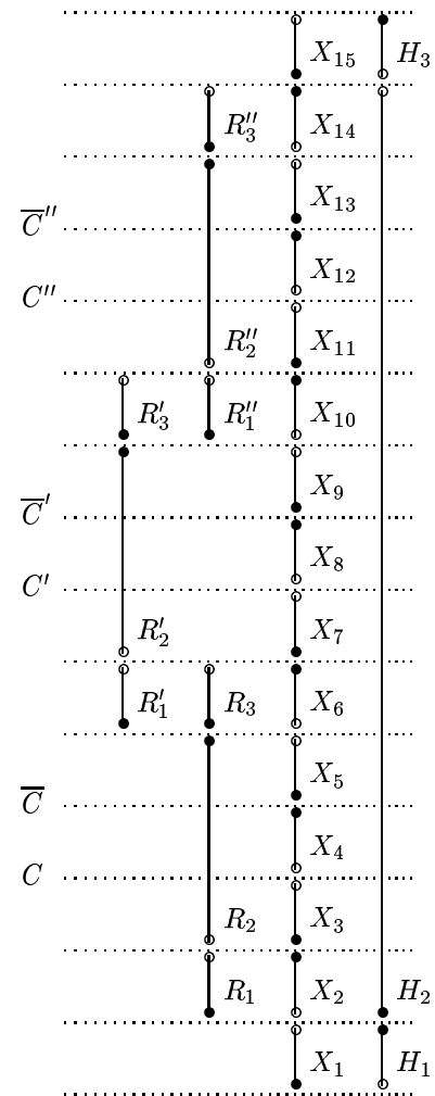
Figure 1: Representing a variable: Vertical lines indicate intervals associated with individual genes. The \bullet and \circ symbols indicate the two optimal placements of genes. C, C', C'' indicate gaps between consecutive genes associated with a clause containing the unnegated variable, \bar{C}, \bar{C}', \bar{C}'' gaps for clauses containing the negated variable.
