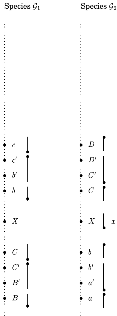
Figure 3: Depth 2 gene arrangement: a satisfied clause allows an additional pairing to be made, namely (X, C) . If the \Gamma(x) containing a, a', b', b had its other optimal arrangement, then we could choose between (X, C) and (X, b) . (Gene x prevents both pairings simultaneously.)
